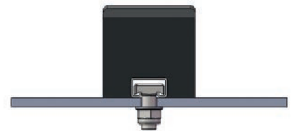
REMASLIDE ATEX with TT-Fastening Unit type IV
