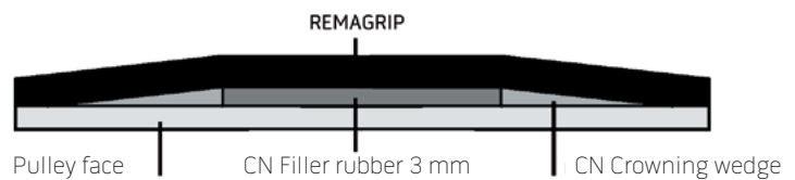
Pulley crowning with CN Crowning wedge and CN Filler rubber
